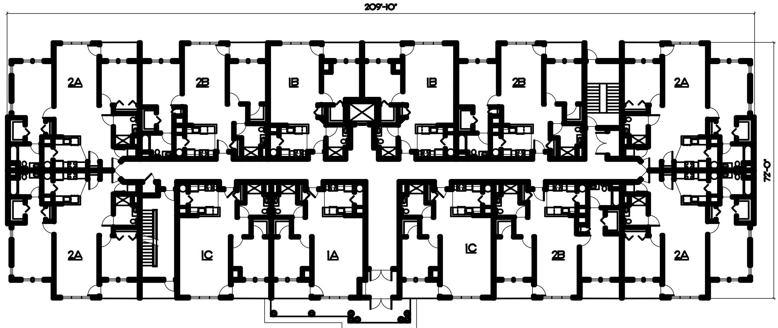
Building D First Floor Plan (36 Unit Building)
