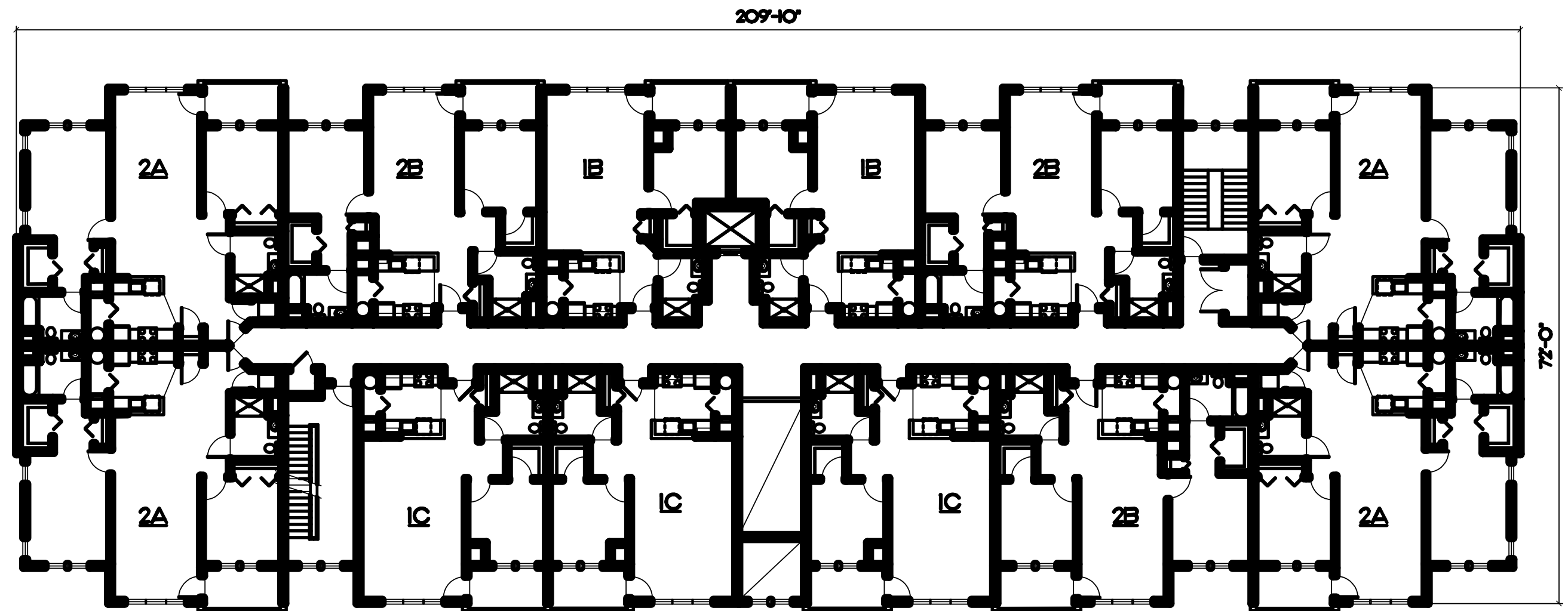
Building D Second Floor Plan (36 Unit Building)
